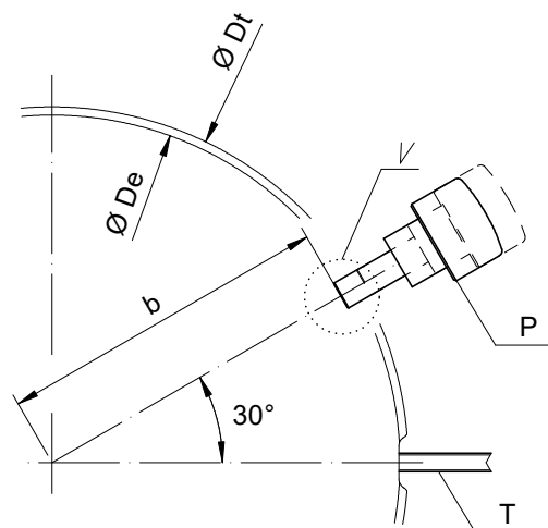
Detail V
